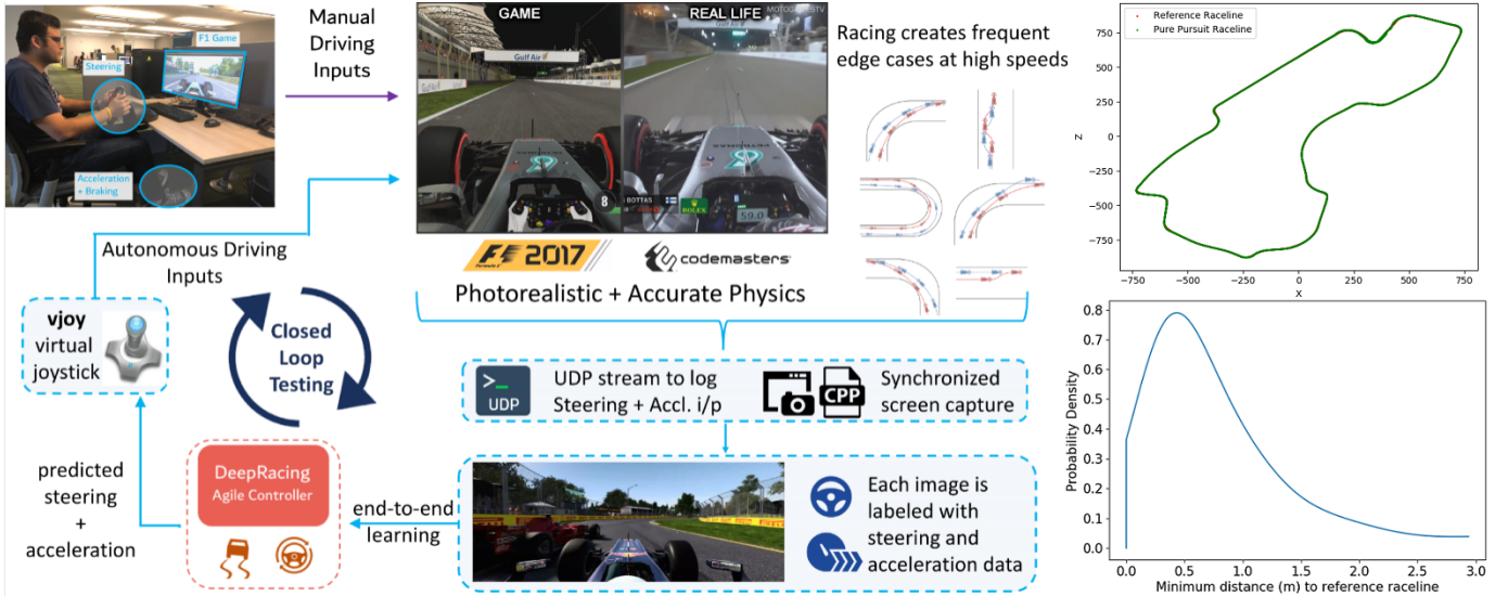
Fig. 1. DeepRacing uses the Formula One Codemasters game as a virtual testbed for training and closed-loop testing for our autonomous racing deep neural network - AdmiralNet. This is the first time the highly photo-realistic and high fidelity physics engine enabled game has been used as a simulation environment without cracking and tweaking any game engine code.
