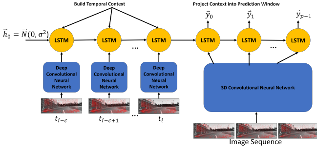
Fig. 2. AdmiralNet architecture
