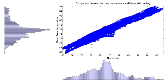
Figure 14: Scatter plot between the mean temperature measurement (y-axis) and the thermostat reading (x-axis). The spread of a data indicates the bias between the thermostat and the mean temperature measurement.
