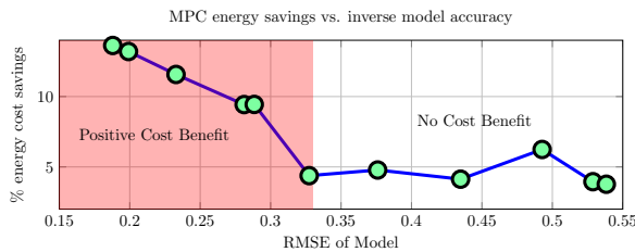
Figure 10: MPC performance for models of different degrees of accuracy.
